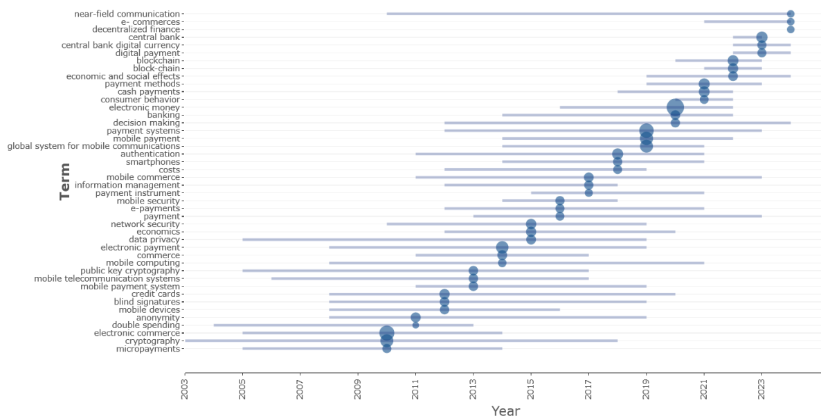
Figura 8 - Trend topics
